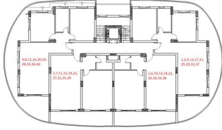
Tip Kat Plan
